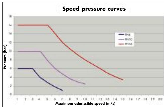
Fig. 4 Speed - pressure curves.
