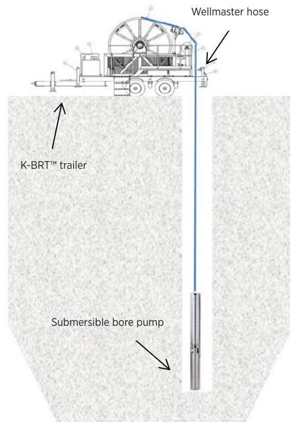
K-BRT™ Trailer retrieval of submersible pump
