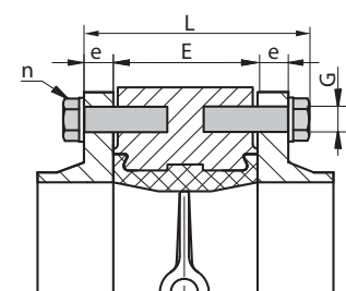
Version B
