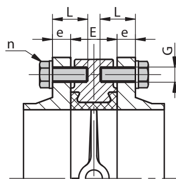
Version B
